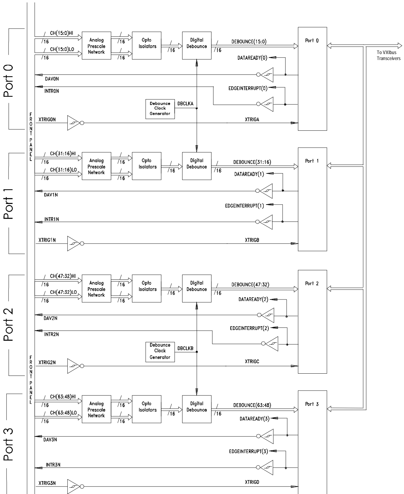
Figure 1-1. Agilent E1459A 64-Channel Isolated Digital Input/Interrupt Block Diagram
