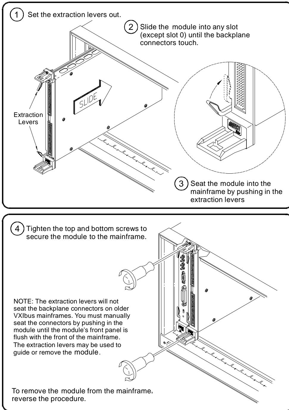
Figure 1-8. Installing the Agilent E1459A in a VXIbus Mainframe
