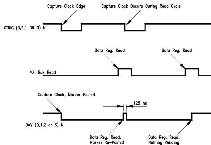
Figure 1-4. DAV Timing
