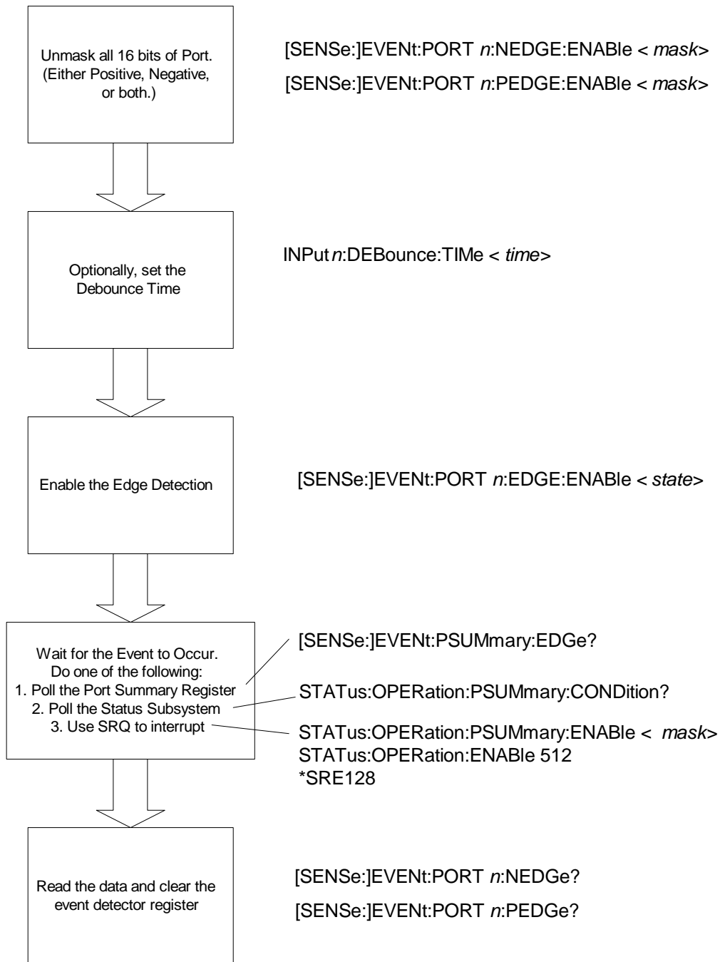
Figure 2-1. Agilent E1459A Edge Event Detection Flowchart
