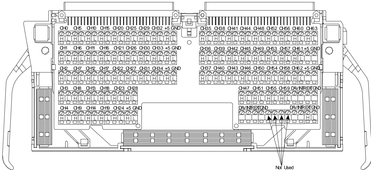
Figure 1-9. Agilent E1459A Standard Screw-type Terminal Block
