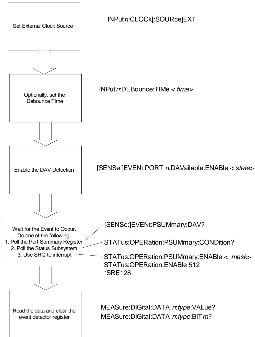
Figure 2-2. Agilent E1459A Data Available Event Detection Flowchart
