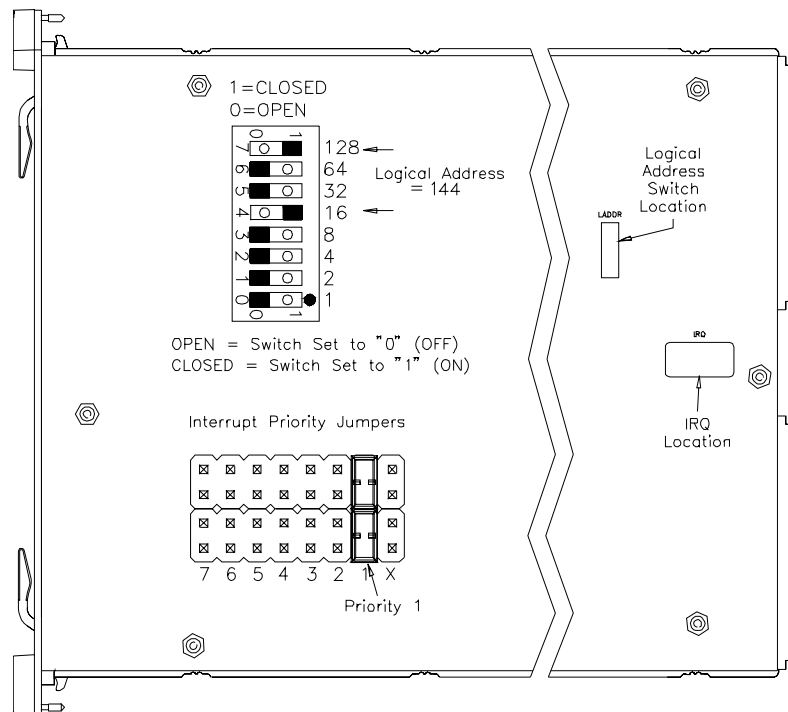
Figure 1-5. Agilent E1459A Logical Address Switch and IRQ Jumper Locations
